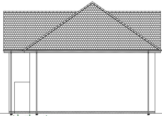
Side Elevation
