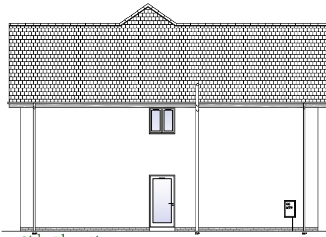
Side Elevation
