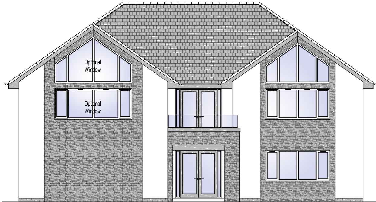
Front Elevation
